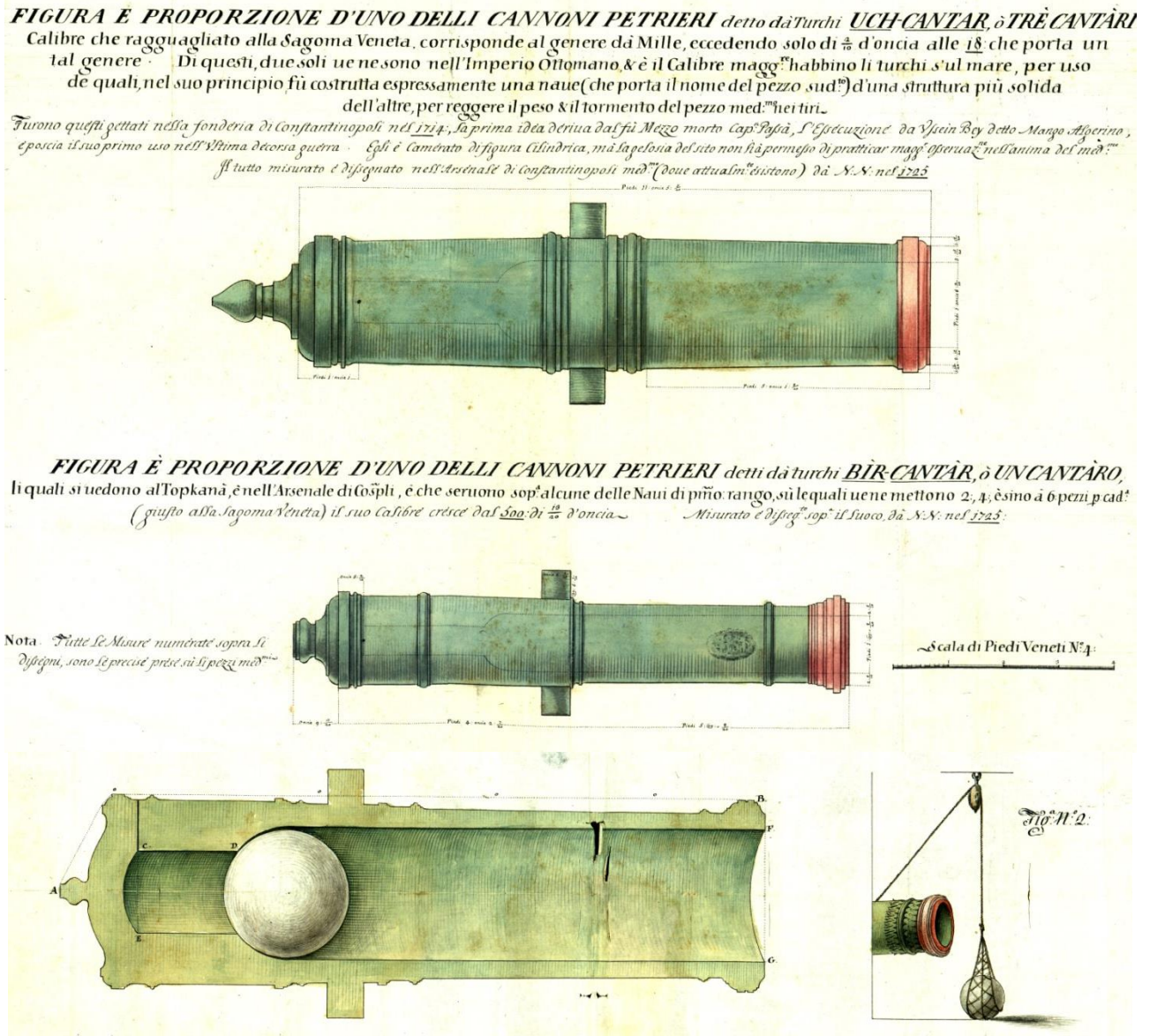
Figure 3. Scale comparison of a 3-kantar and a 1-kantar barrel (above) and the cutaway view of a 3-kantar barrel; together with the sling and pulley system to handle the enormous 336 pound marble ball (below) These drawings are part of a Venetian spy report from 1725
